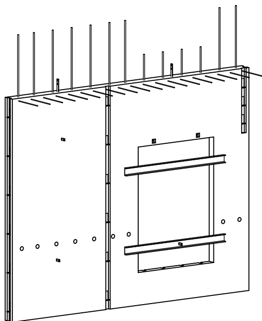
6 3D VIEW
