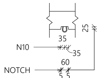
NOTCH DETAIL-A
